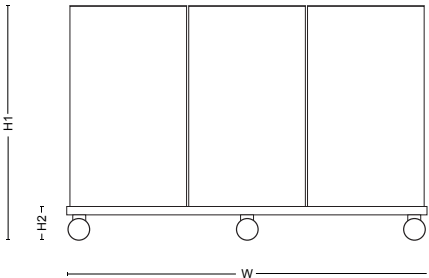
Arkad Trio stand with casters H1: 787mm, 31" H2: 87 mm, 3.4" W: 1250 mm, 49.2" D: 425 mm, 16.7"
