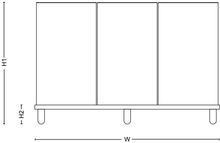
Arkad Trio stand H1: 820 mm, 32.3" H2: 120 mm, 4.7" W: 1250 mm, 49.2" D: 425 mm, 16.7"
