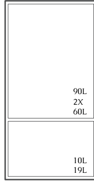
X6/12-90 & 6/12-60 H: 1161 mm, 45,7" W: 615 mm, 24,2" D: 605 mm, 23,8"
