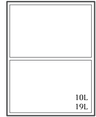
X6/7-19 H: 781 mm, 30,7" W: 615 mm, 24,2" D: 605 mm, 23,8"
