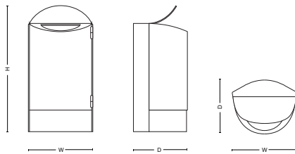
Captin Weight: 35 kg, 77,2 lbs H: 1023 mm, 40.3" W: 525 mm, 20.7" D: 442 mm, 17.4"
