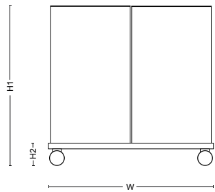
Arkad Duo stand with casters H1: 787mm, 31" H2: 87 mm, 3.4" W: 838 mm, 33" D: 425 mm, 16.7"
