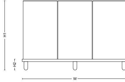
Arkad Trio stand H1: 820 mm, 32.3" H2: 120 mm, 4.7" W: 1250 mm, 49.2" D: 425 mm, 16.7"
