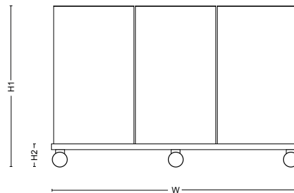
Arkad Trio stand with casters H1: 787mm, 31" H2: 87 mm, 3.4" W: 1250 mm, 49.2" D: 425 mm, 16.7"
