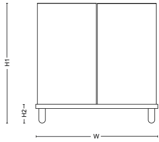
Arkad Duo stand H1: 820 mm, 32.3" H2: 120 mm, 4.7" W: 838 mm, 33" D: 425 mm, 16.7"
